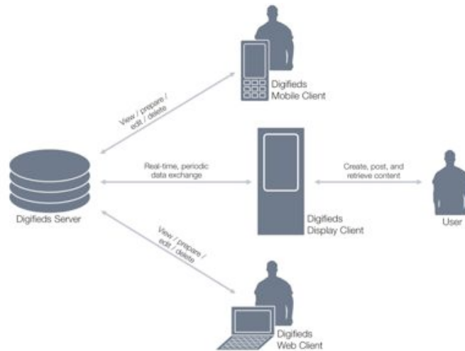
Fig. 9. Digifieds conceptual system architecture: The Digifieds server stores and maintains the content. Mobile clients, display clients, and web clients can connect to the server in order to exchange content.
